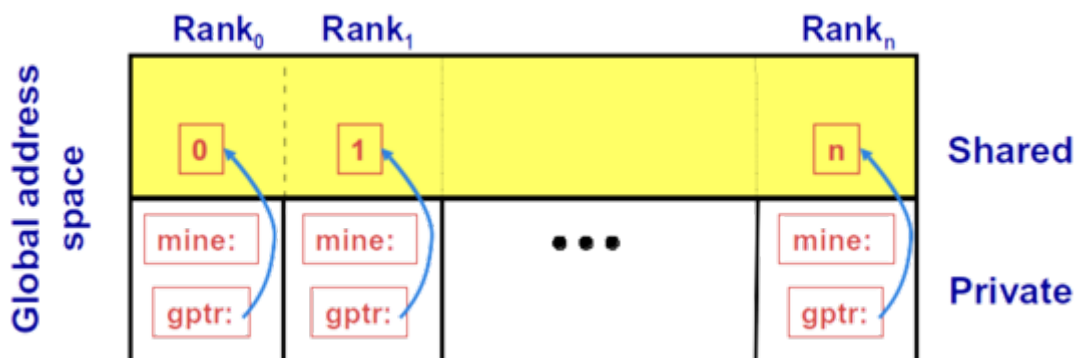
Figure 2: Figure 2. Global pointers.
