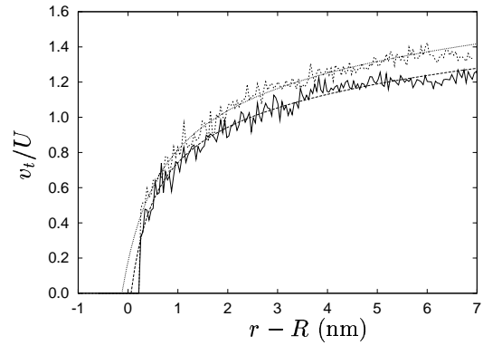
Figure 6: The time average tangential component of the streaming velocity for the flow past an array of carbon nanotubes. The profiles are sampled from section II and V and compared with equation (3) for the 1.25 nm tube: —: measured; - -: fit and the 2.50 nm tube: · · ·: measured; · · ·: fit.
