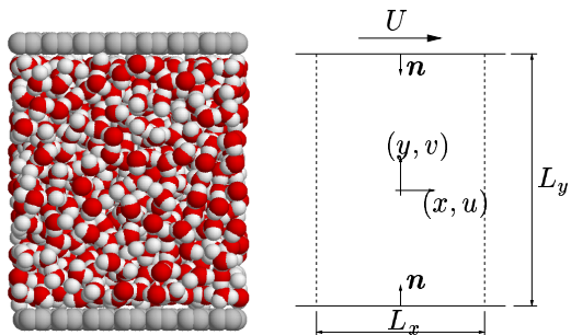
Figure 1: Sketch of the planar Couette flow problem. L_x and L_y denote the length of the unit cell in the streamwise ( x ) and wall normal direction ( y ). The upper wall is forced to move with a constant velocity ( U ) and periodic boundary conditions are enforced in the streamwise and the spanwise ( z ) directions.
