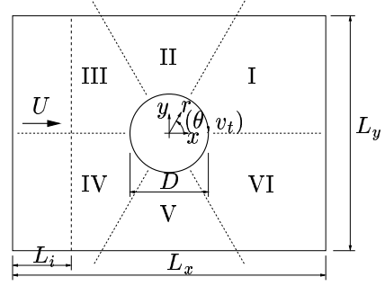
Figure 4: Sketch of the carbon nanotube-water system. D denotes the diameter of the carbon nanotube, L_x the size of the system in the streamwise direction, and L_y and L_z the height and width, respectively. The velocity of the center of the mass of the water molecules contained in the “inlet” region ( L_i ) of the computational box is fixed to the desired value ( U ).
