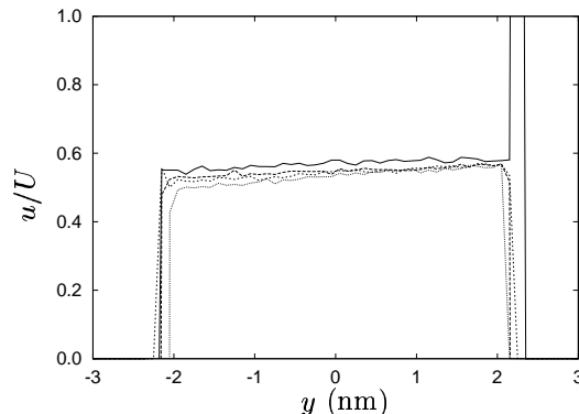
Figure 2: Time average streaming velocity profiles in a Couette flow as function of the system pressure: — : 10 bar (case 1); - - : 200 bar (case 2); - · - : 500 bar (case 4); ··· : 1000 bar (case 4).
